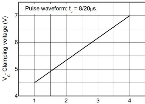
I_{PP} - Peak pulse current (A)
