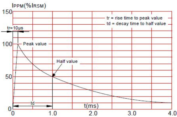
FIG.3: Pulse waveform
