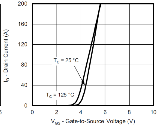
Transfer Characteristics
