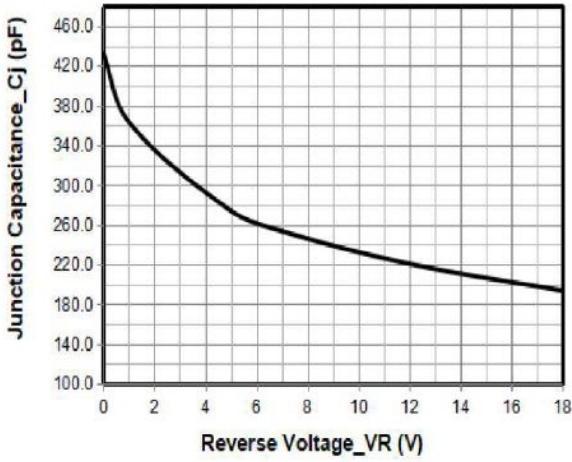
Novction Capacitance vs. Reverse Voltage
