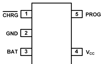
SOT23-5 (Top View)
